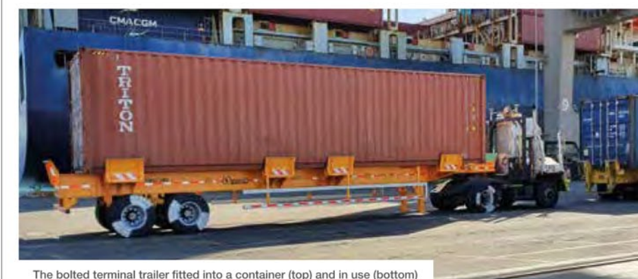
The bolted terminal trailer fitted into a container (top) and in use (bottom)
